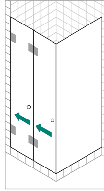
APPLICATION AQUAFOLD 3 CORNER APPLICATION OF SINGLE FOLDING DOOR WITH ONE FIXED GLASS PANEL
